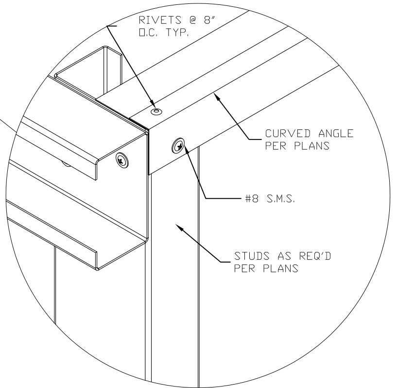
D SOFFIT WITH CURVED ANGLE DETAIL XX N.T.S.
