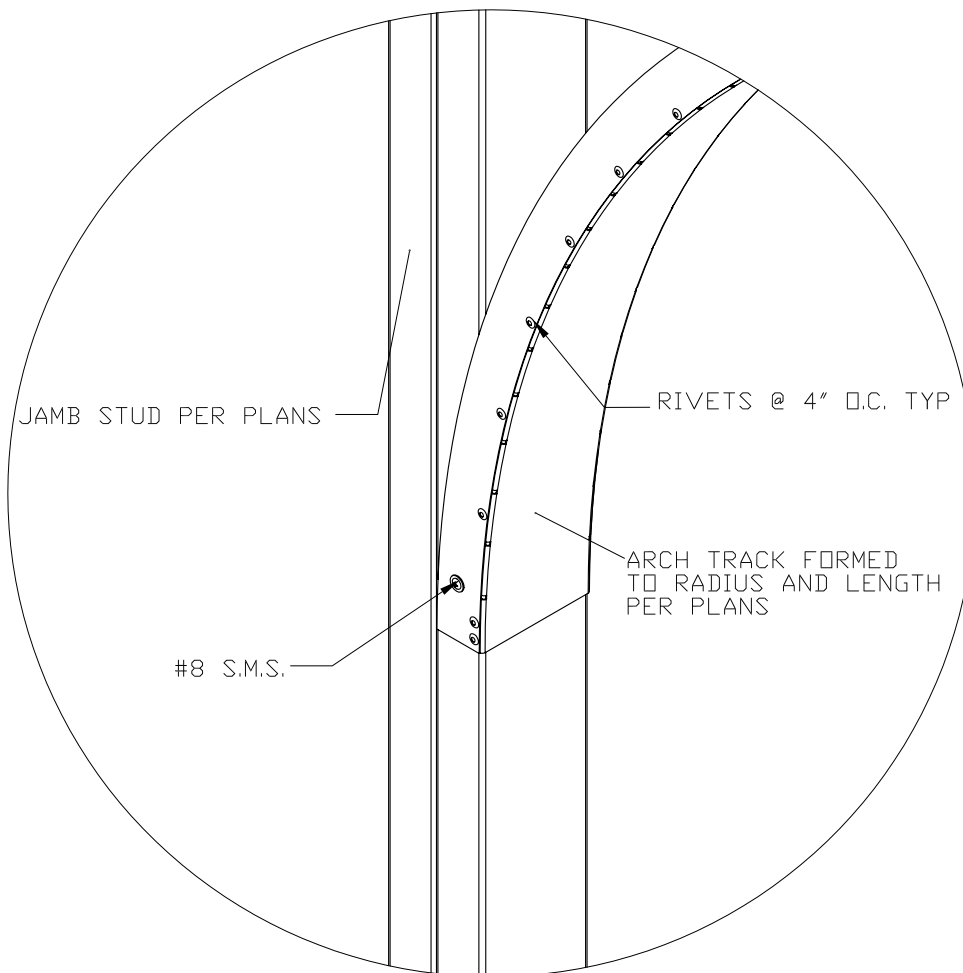
B ARCHED TRACK ENTRY DETAIL XX N.T.S.
