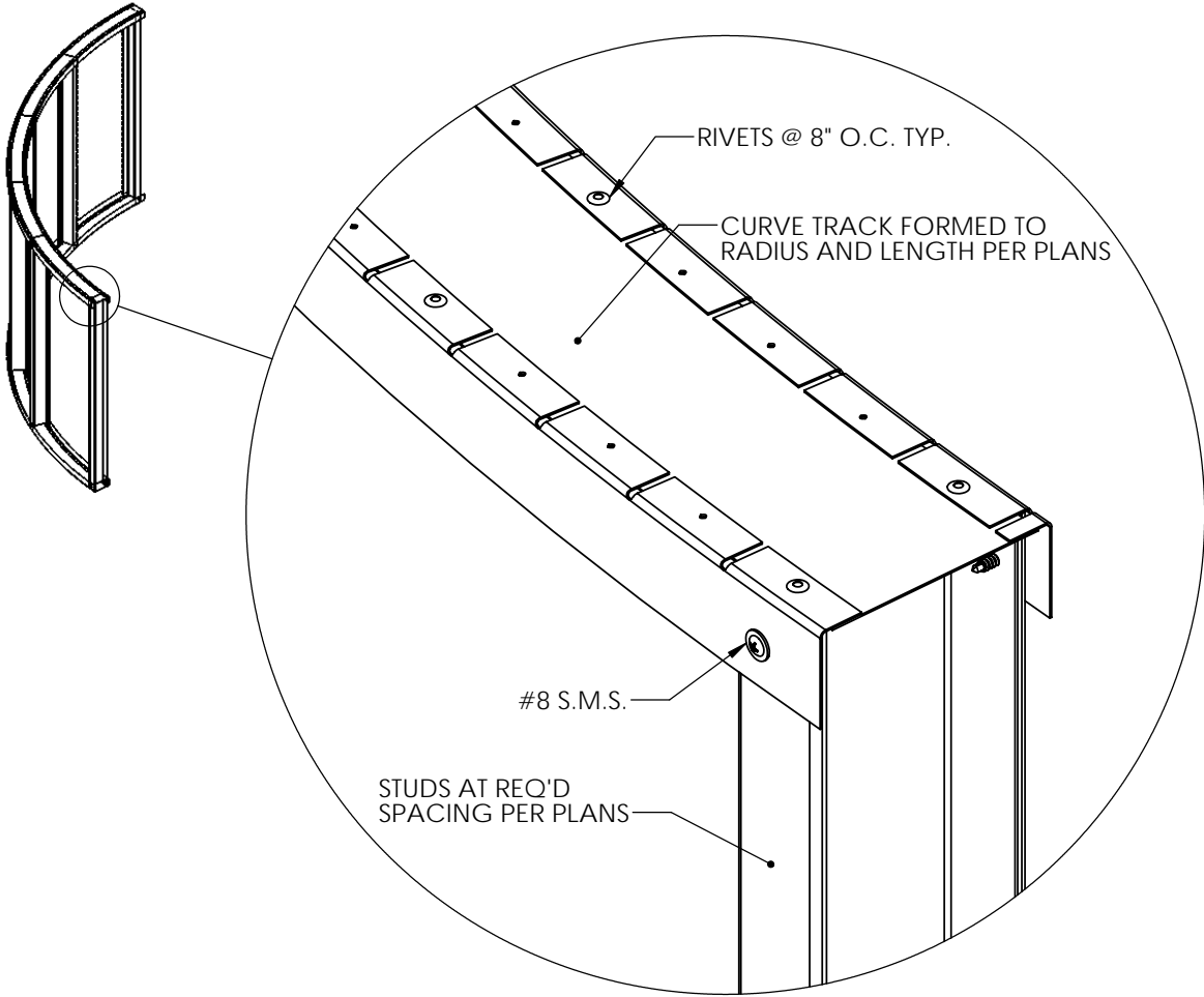
A XX CURVED WALL TRACK DETAIL N.T.S.
